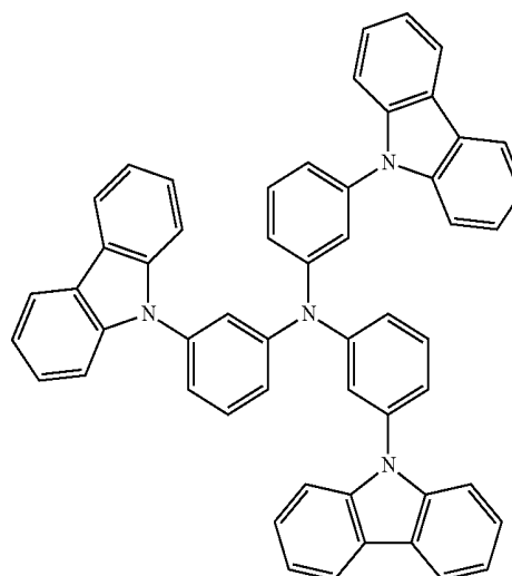
[Formula 6]
