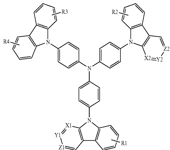
[Formula 9]
