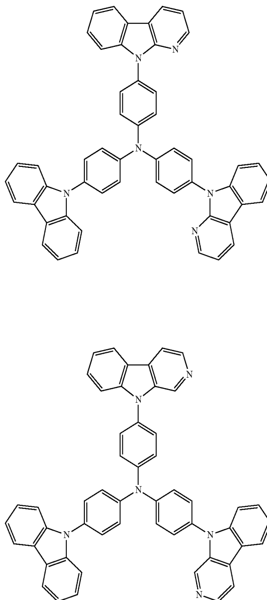
[Formula 10]
