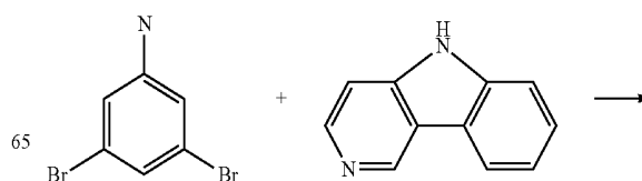
[Reaction Formula 3] 60
