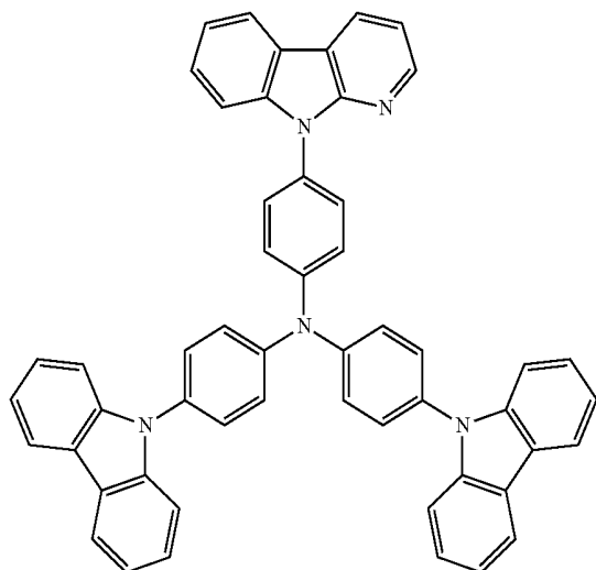
[Formula 12]
