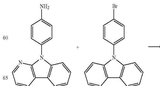
[Reaction Formula 17]
